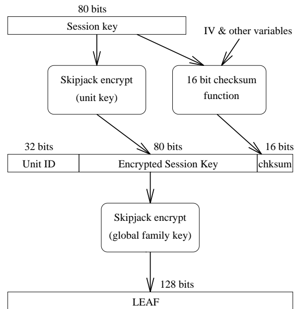
Figure 1: LEAF Structure
